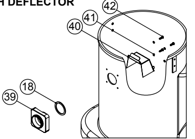
WET USE DIE-CAST FLANGE WITH DEFLECTOR
