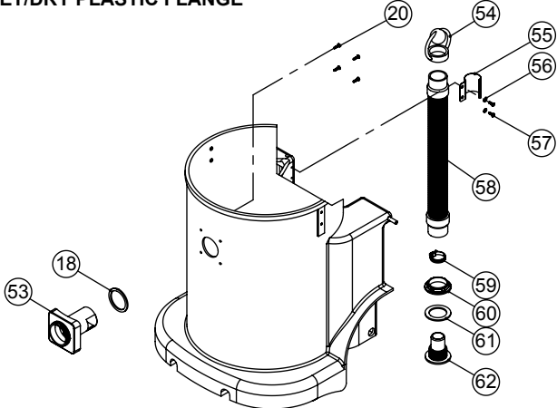
LARGE DUMP HOSE WET/DRY PLASTIC FLANGE
