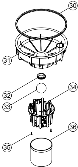
FLOAT ASSEMBLY
